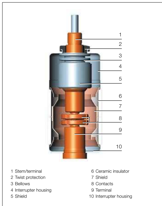
Vacuum interrupter
